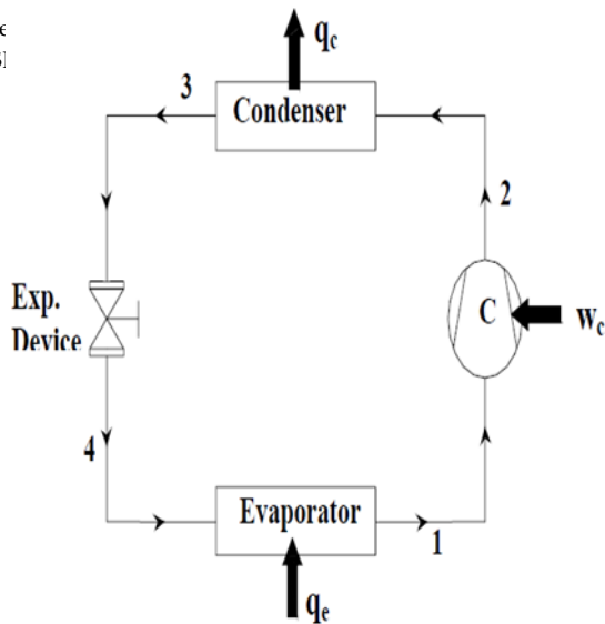
Fig 1- vapour compression system
